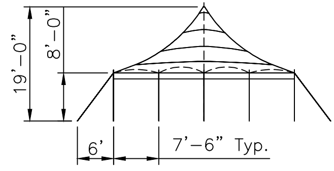
End View
