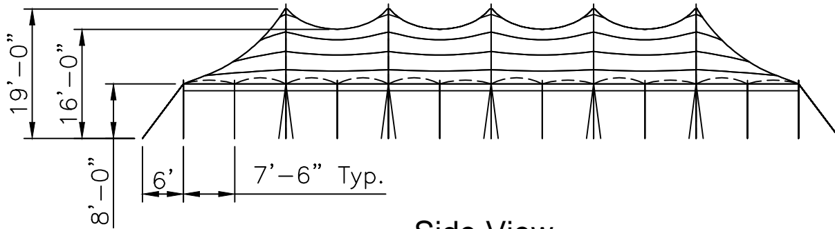
Side View
