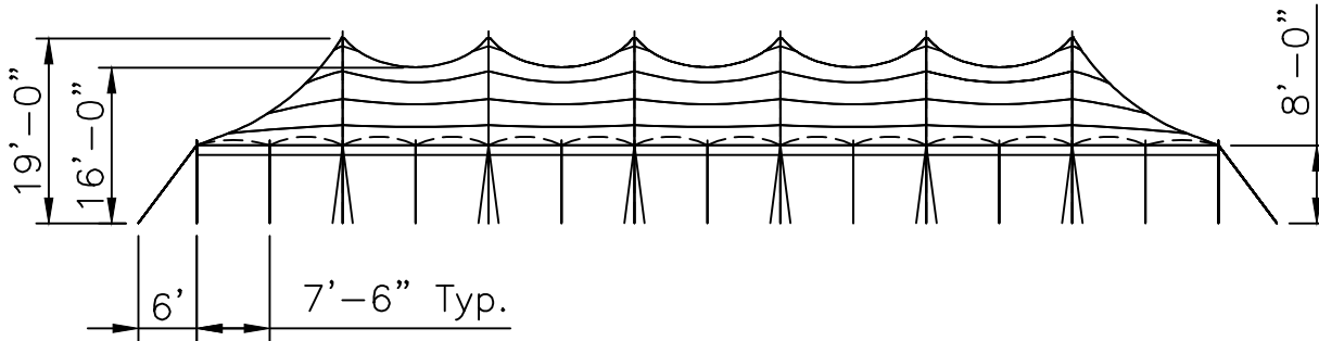
Side View
