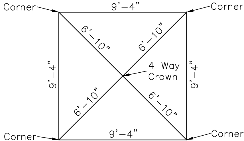
Frame Top View
